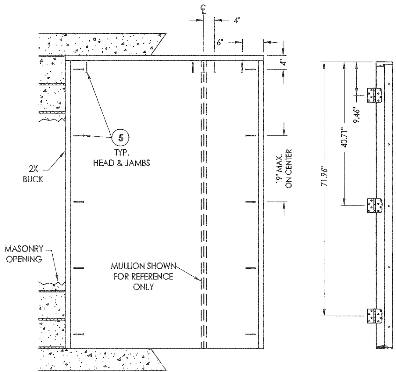
BUCK ANCHORING
