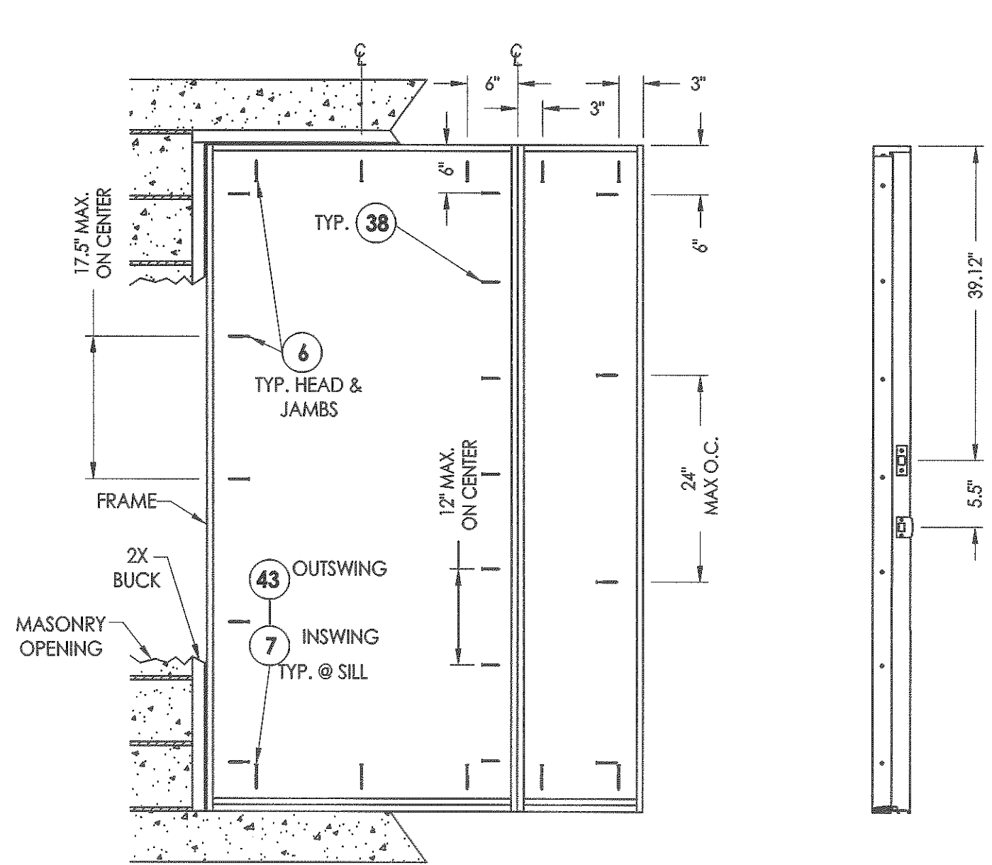
FRAME ANCHORING Masonry 2X buck construction
