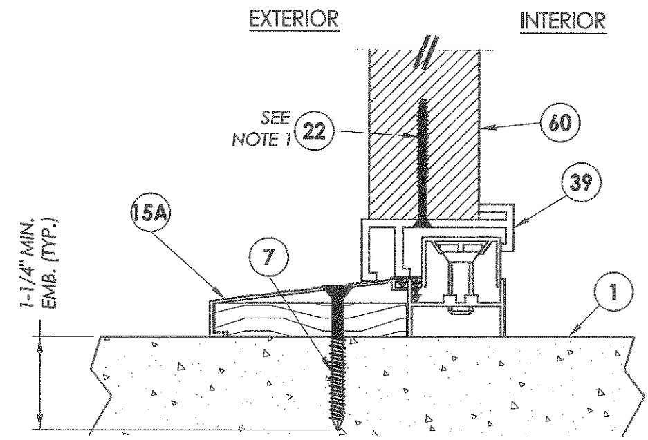
2 VERTICAL CROSS SECTION 6 Shown w/1X sub-buck
